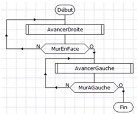
Programme Principal
